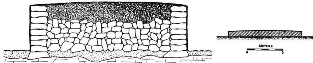
a, Cross section of Sacbe showing mode of construction. Smaller diagram to the right shows the construction in true proportion.
